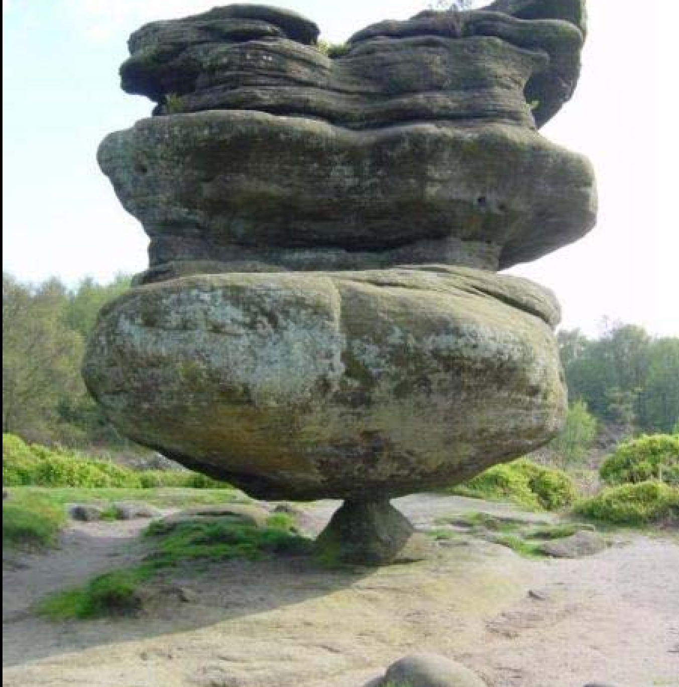
Brimham Rock - England, UK
